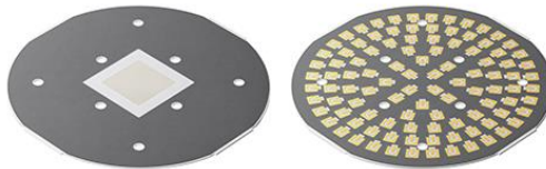
Flip chip substrate for QPU chip
